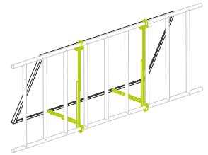
Balcony mounting system
